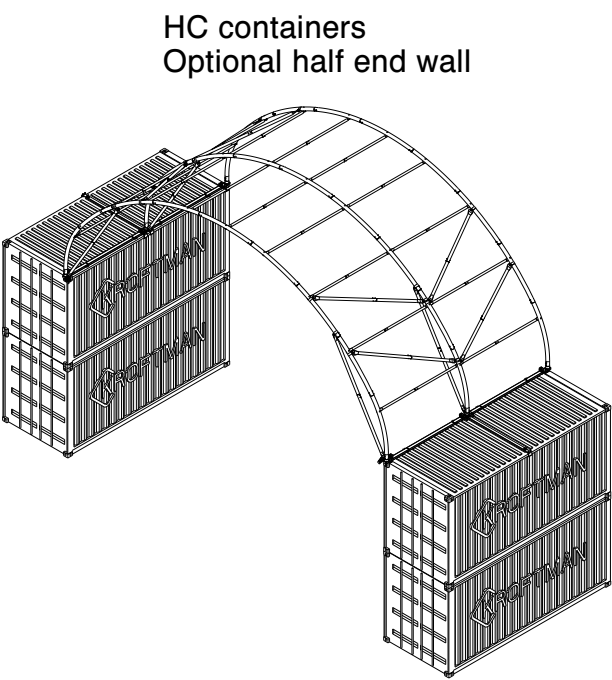
SCALE 1:200
