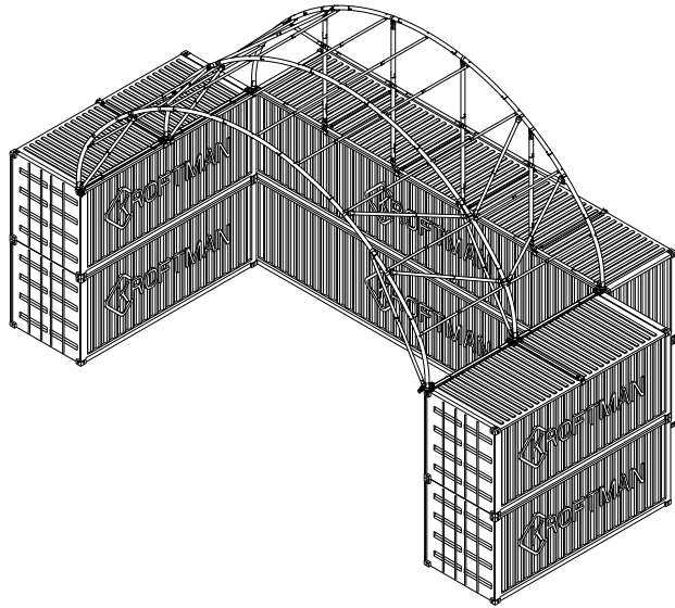
SCALE 1:200
