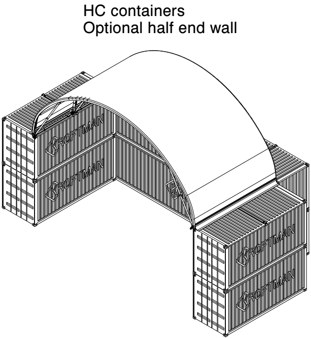
SCALE 1:200
