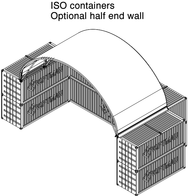
SCALE 1:200
