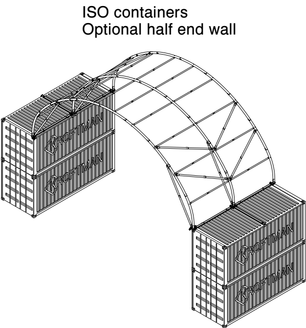
SCALE 1:200
