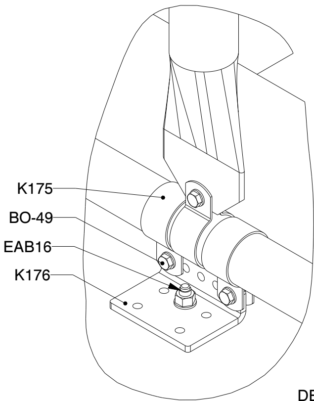
DETAIL F SCALE 1:5 2xM12 / 1xM16
