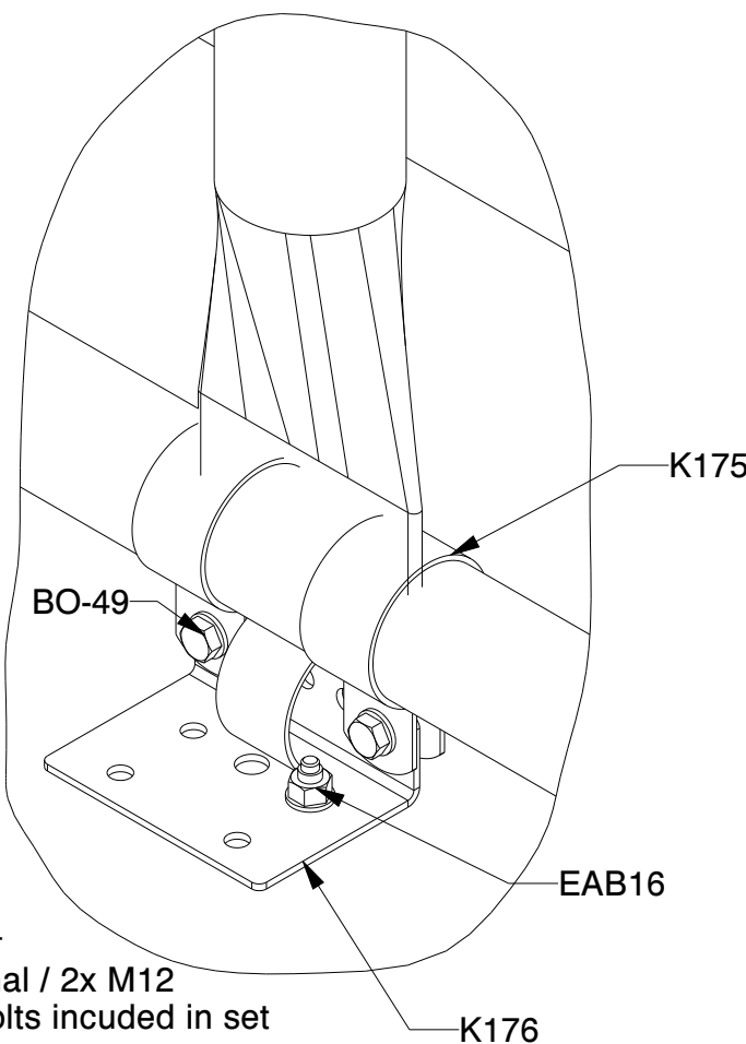
DETAIL E SCALE 1:4
